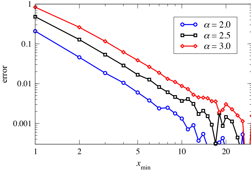
FIG. B.1. The error on the estimated scaling parameter \hat{\alpha} that arises from using the approximate MLE for discrete data, Eq. (3.7), for \alpha = 2, 2.5, and 3 (for 1000 repetitions), as a function of x_{\min} . The average error decays as O(x_{\min}^{-2}) and becomes smaller than 1% of the value of \alpha when x_{\min} \gtrsim 6 .
