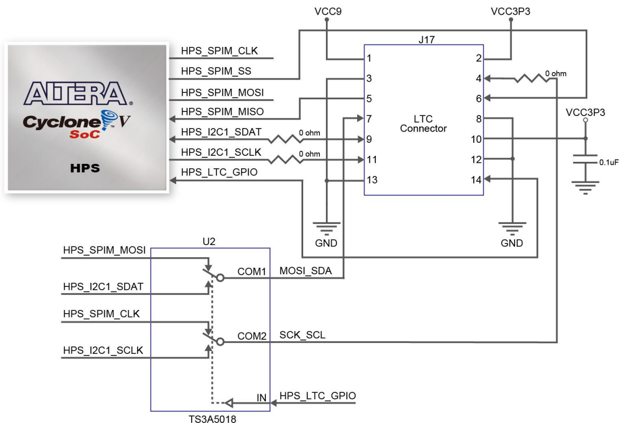
Figure 3-26 Connections between the HPS and LTC connector
