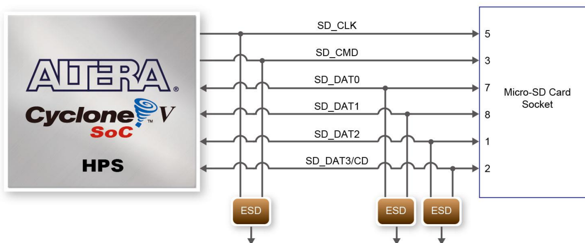
Figure 3-23 Connections between the FPGA and SD card socket
