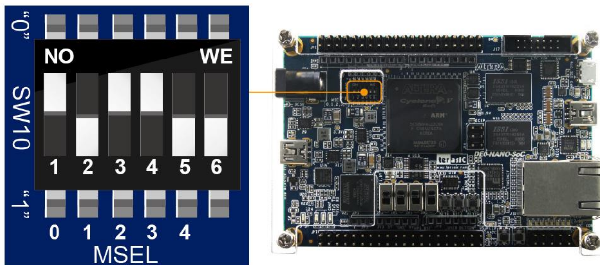
Figure 3-1 DIP switch (SW10) setting of Active Serial (AS) mode at the back of DE0-Nano-SoC board
