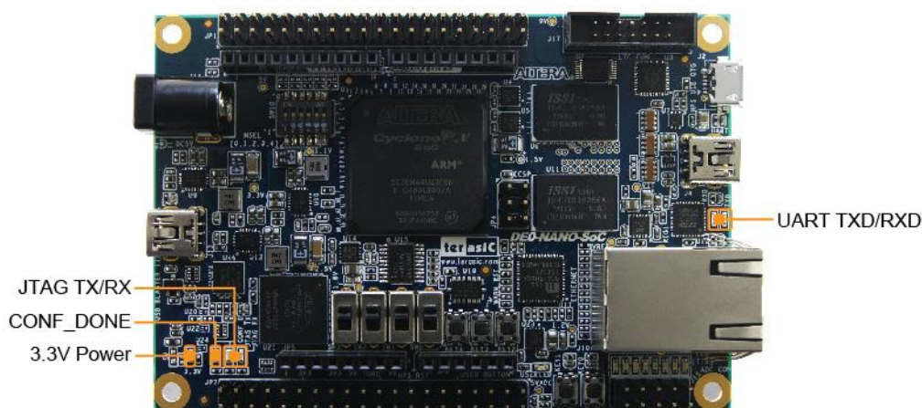
Figure 3-10 LED Indicators on DE0-Nano-SoC
