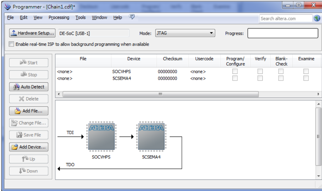
Figure 3-5 FPGA and HPS detected in Quartus programmer
