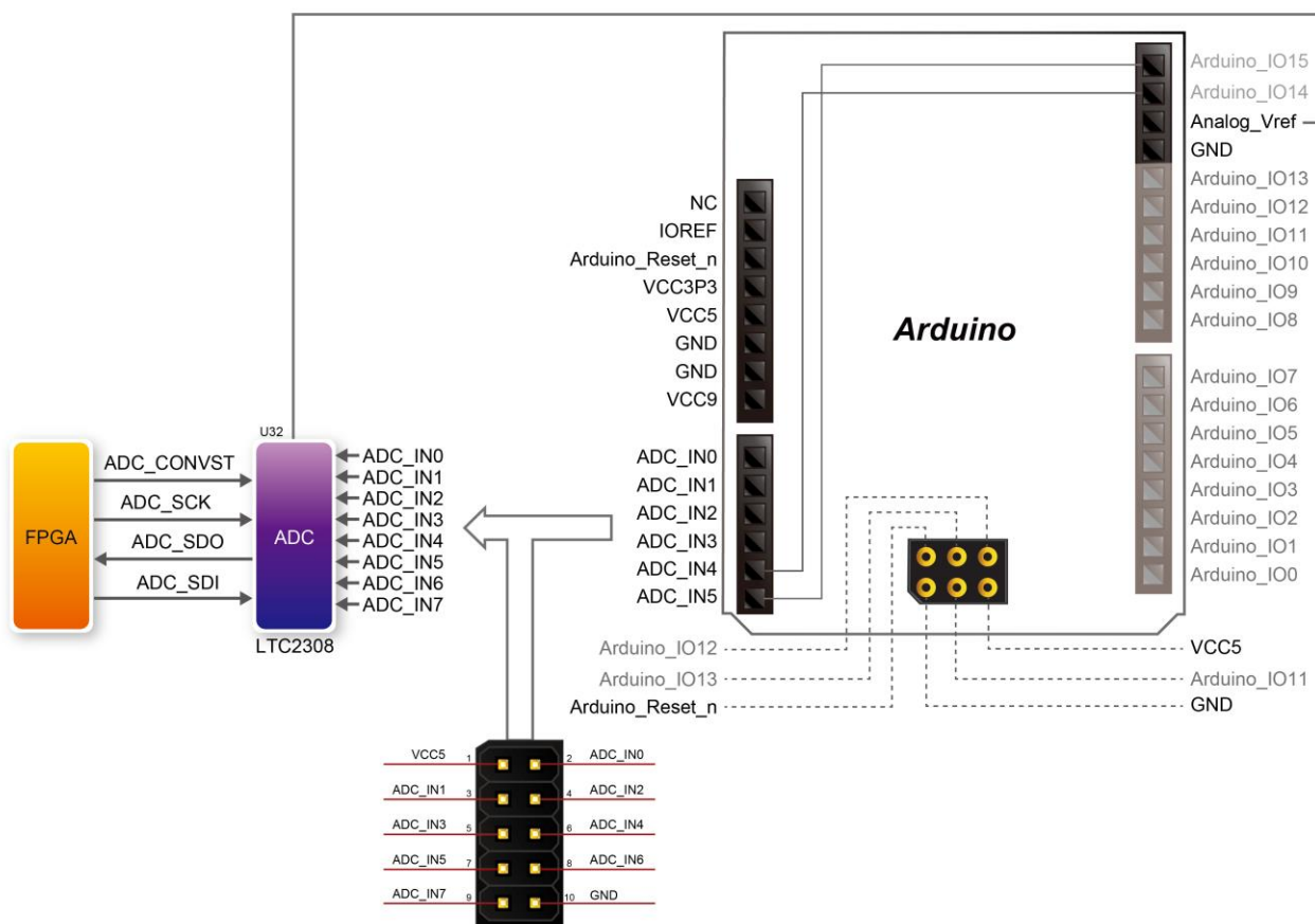
Figure 3-20 Connections between the FPGA, 2x5 header, and the A/D converter
