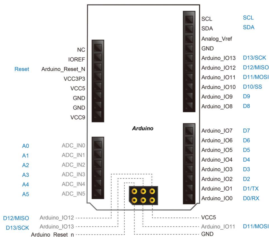
Figure 3-18 lists the all the pin-out signal name of the Arduino Uno connector. The blue font represents the Arduino pin-out definition.
