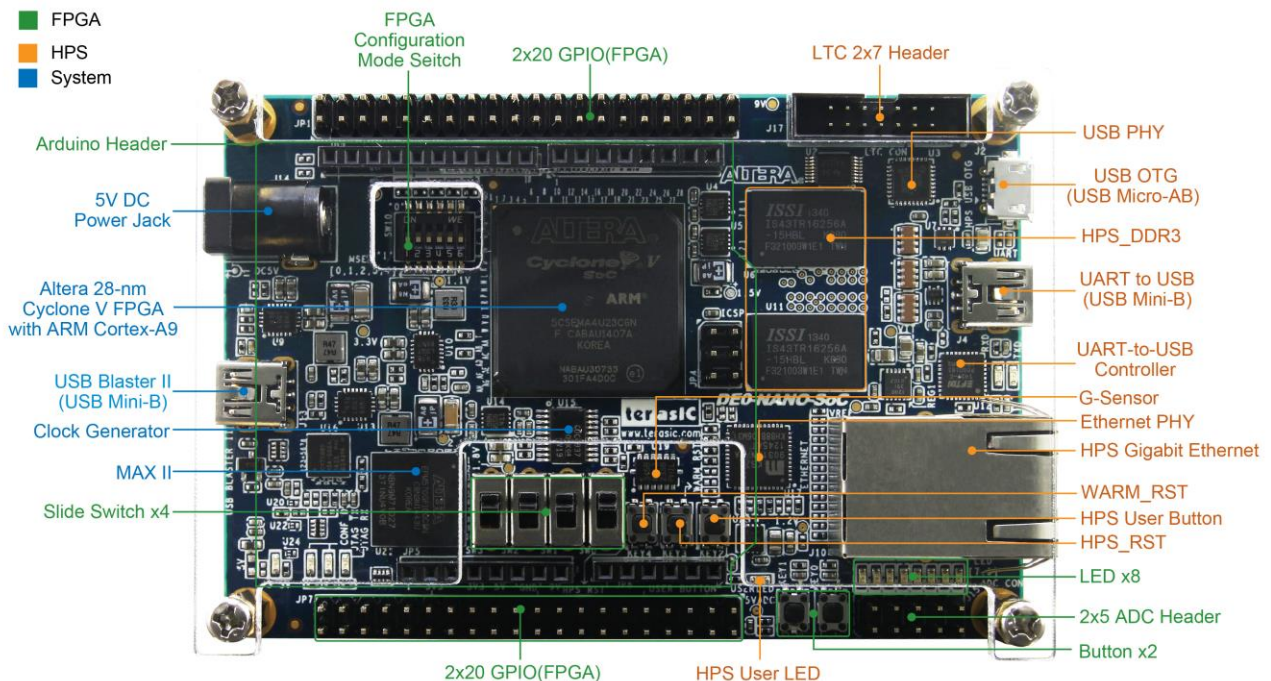
Figure 2-1 DE0-Nano-SoC development board (top view)
