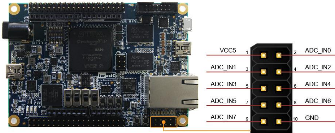
Figure 3-19 Signals of the 2x5 Header
