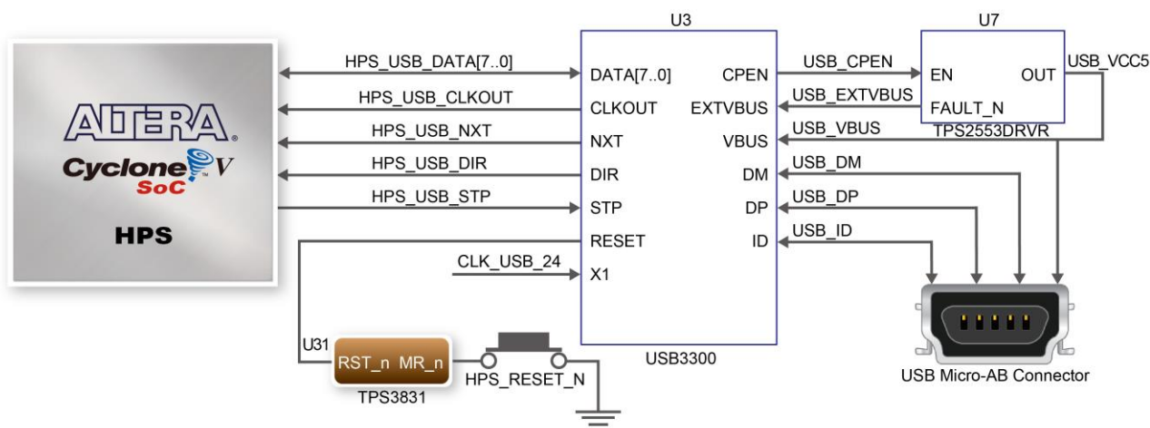
Figure 3-24 Connections between the HPS and USB OTG PHY
