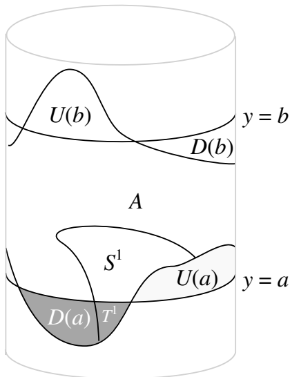
Figure 5: Upward and downward moving sets for a map on the cylinder.
