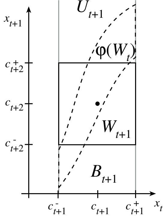
Figure 8: The image of a four dimensional window, W_t under \varphi crosses the window W_{t+1} . We suppress both of the \xi coordinates.
