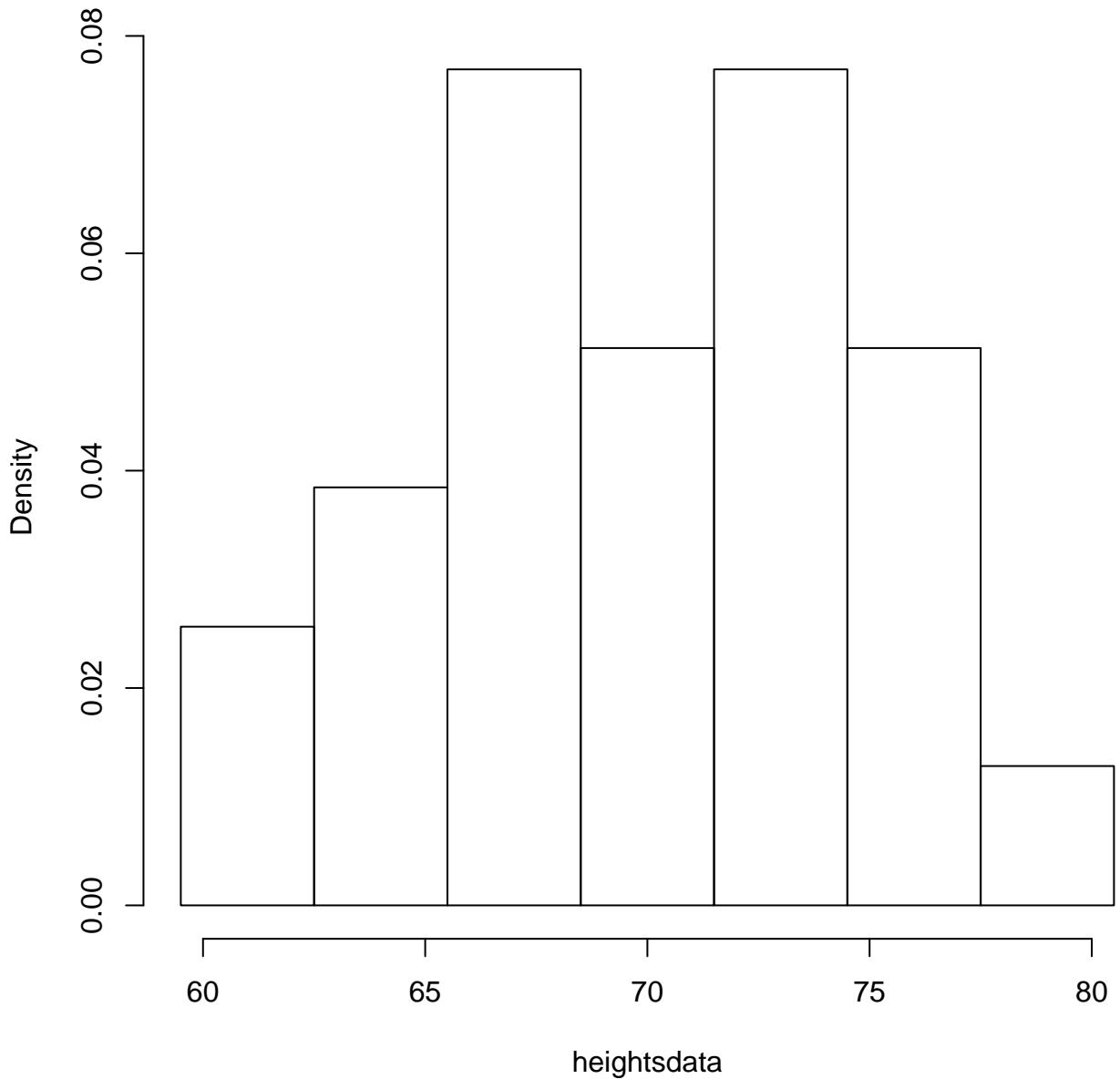
Histogram of heightsdata
