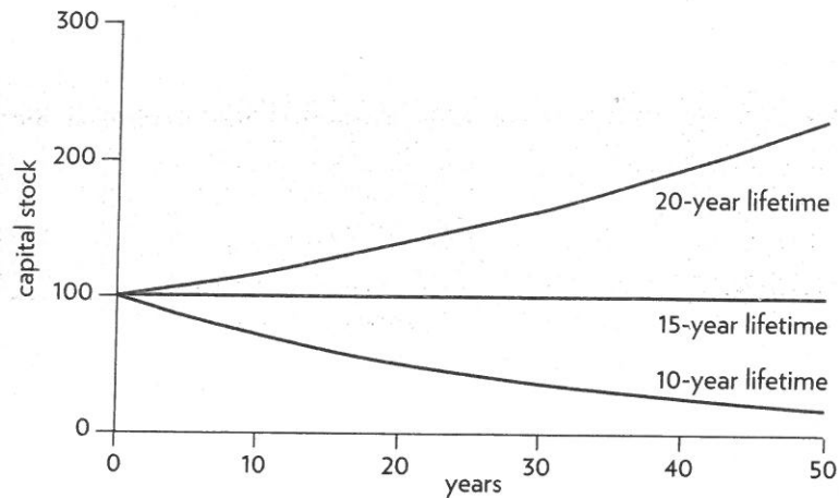
Figure 28. Growth in capital stock with changes in the lifetime of the capital. In a system with output per unit capital ratio of 1:3 and an investment fraction of 20 percent, capital with a lifetime of 15 years just keeps up with depreciation. A shorter lifetime leads to a declining stock of capital.
