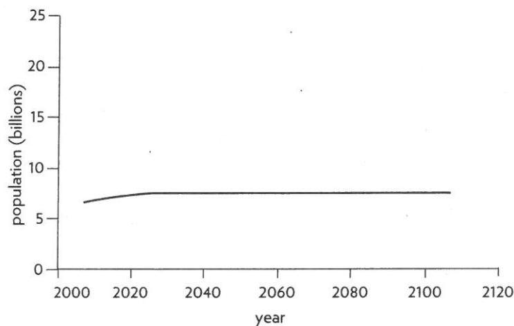
Figure 24. Population stabilizes when fertility equals mortality.
