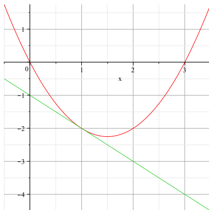
Figure 1: The graph of the function f(x) = x^2 - 3x along with the tangent line at the point x = 1 .
